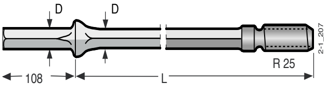
Shank rod, Hex22 - R25
